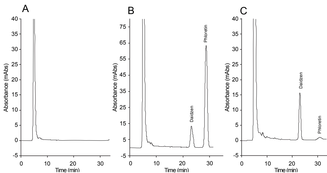
Figure 2: Representative chromatogram of: A) blank serum demonstrating no interfering peaks co-eluted with the compounds of interest; B) rat serum containing IS and phloretin at a concentration of 50 \mu g/mL; C) rat serum containing IS and phloretin with concentration of 0.5 \mu g/mL (LOQ).
